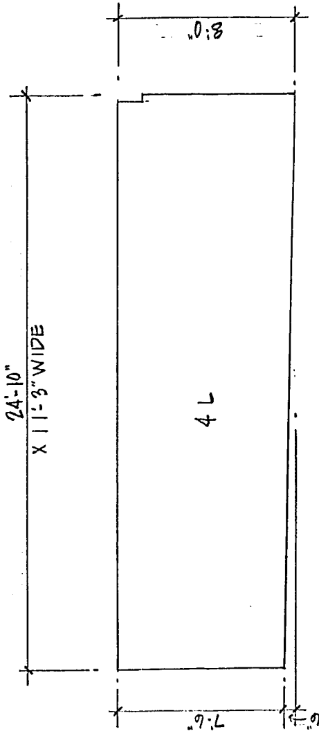
CARPORT SECTION
